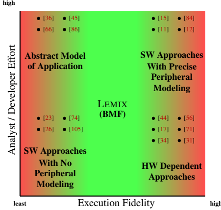
Figure 2: LEMIX in Contrast to Existing Rehosting Approaches.
